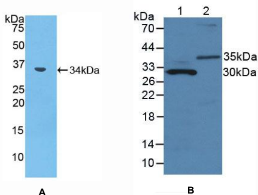
Figure 1. Western Blot
